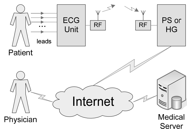
PS – Personal Server; HG – Home Gateway
